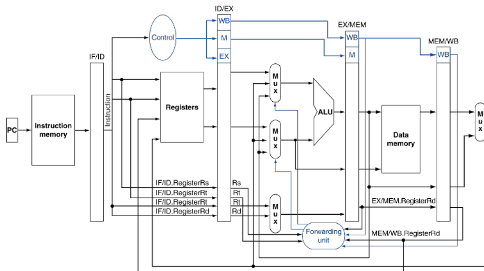
Figure 3: A pipeline MIPS processor. Source: Computer Organization and Design: the Hardware/Software Interface, fifth edition, Morgan Kaufmann Publisher
